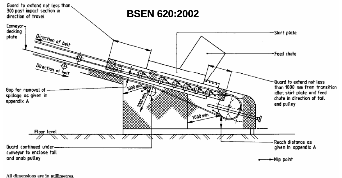
Figure 4. Typical guards at tail end pulley
