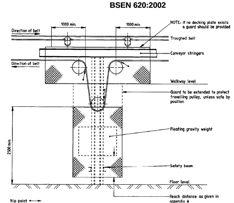
Figure 5. Typical gravity take-up guards
