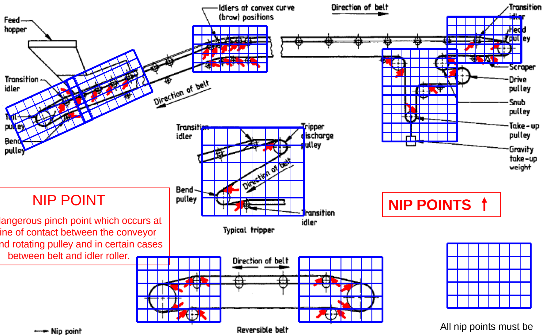
Figure 1 Location of nip points
